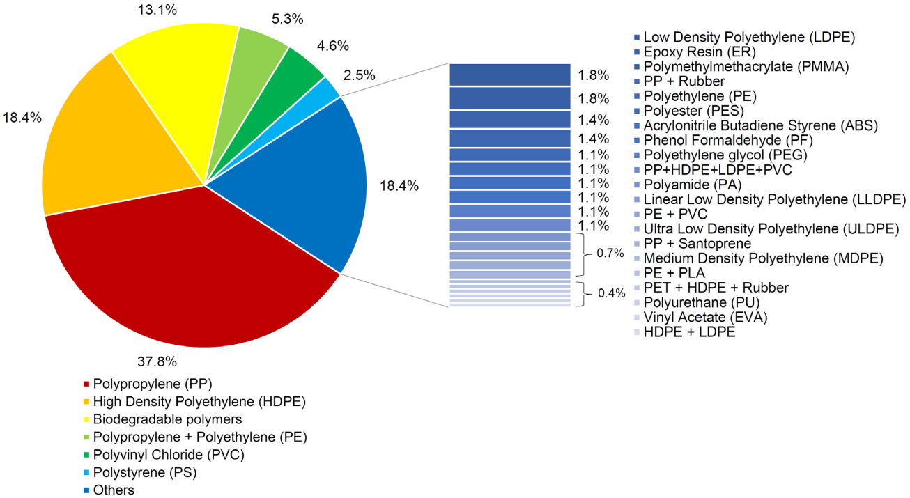
Figure 3: Most used polymers in WPC matrices. Source: The Authors.
