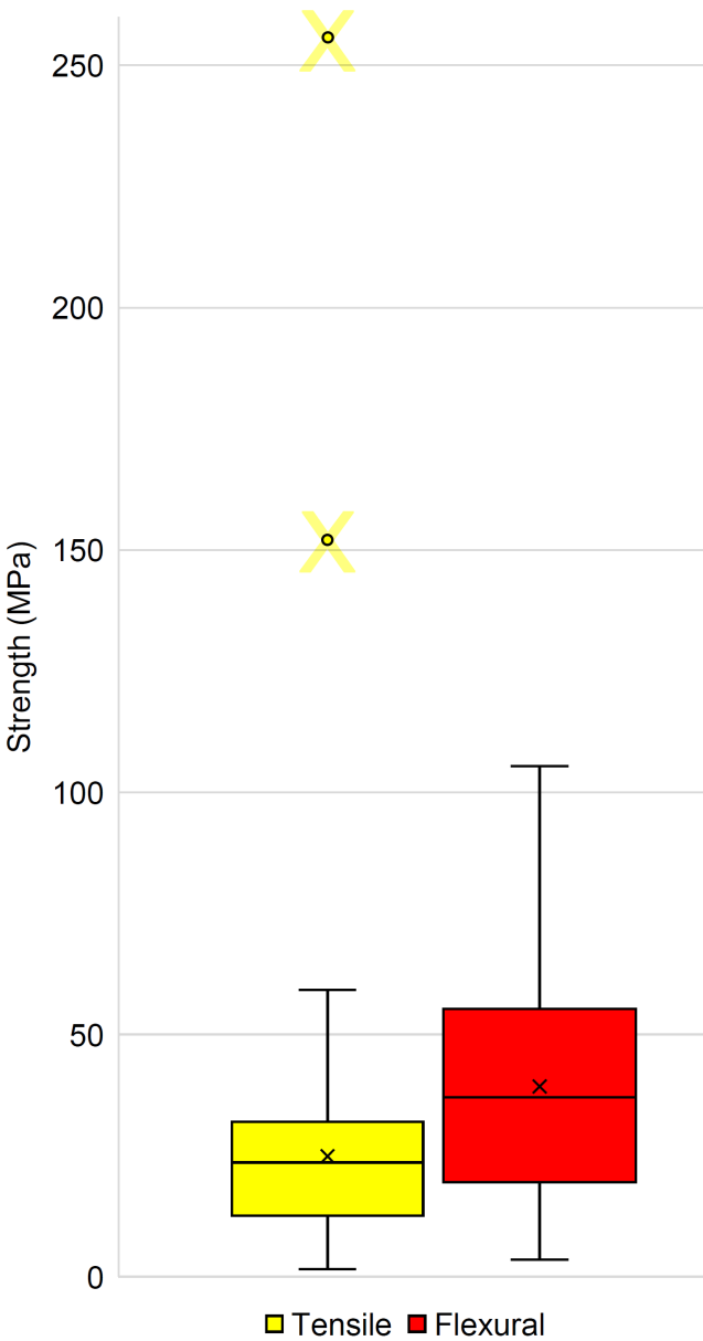
Figure 8: Results of composites subjected to tensile and flexural strength tests. Source: The Authors.
